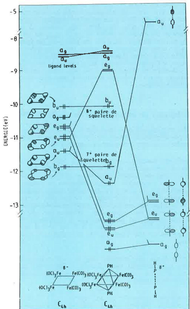
Figure 11. Diagramme orbitalaire de \text{Fe}_4(\text{CO})_{12}(\text{PH})_2 , 33.
