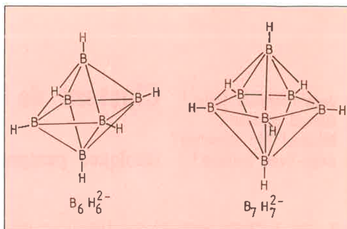
Figure 2. Exemples de clusters boranes closo .
