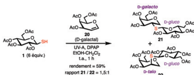
Figure 7 - Addition photo-amorcée de 1-thiosucres aux glycols.
