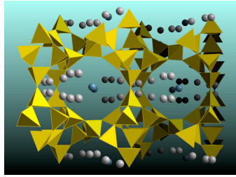
Inorganic nanoporous solid : mineral Stilbite
