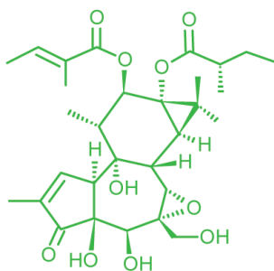
Figure 12 - Le tiglolate de tigilanol.
