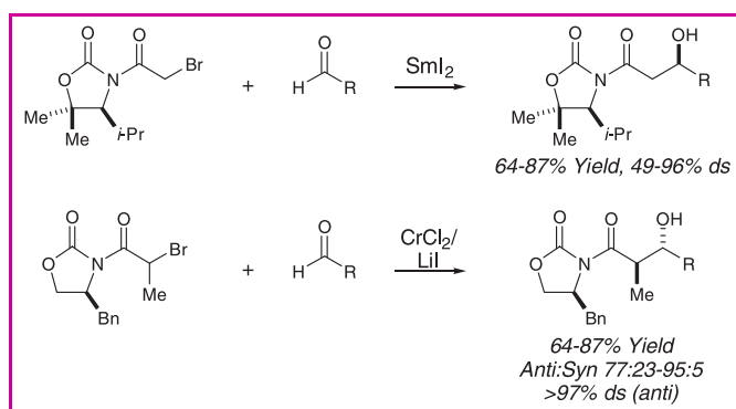
Scheme 7 - Fukuzawa's \text{Sml}_2 (1998) and Wesjohann's \text{CrCl}_2 (1997) Reformatsky reactions.
