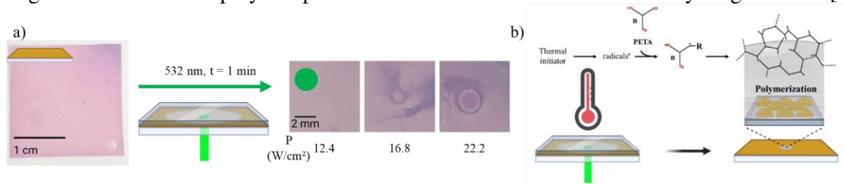
Figure 1: Thermally induced polymerization by thermoplasmonics a) and the associated chemical mechanism b)
